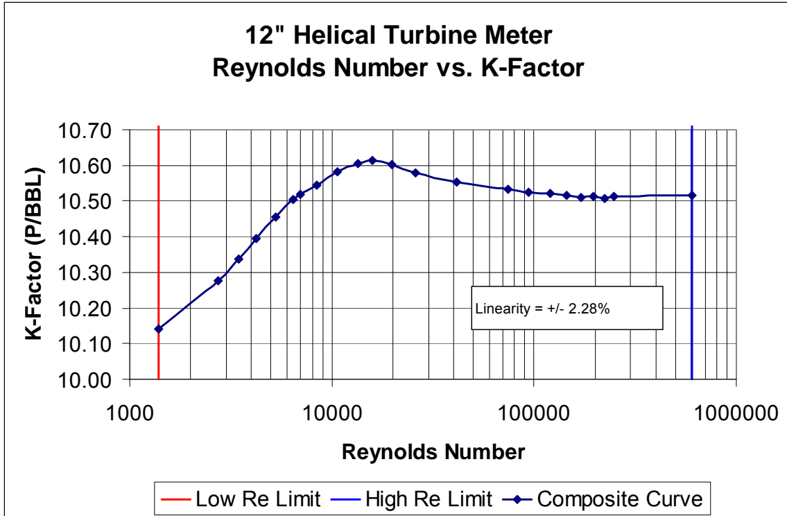
Figure 3 – Universal Performance Curve
