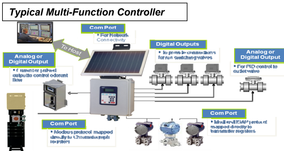
Figure 4. A typical 3 stream flow computer configuration
