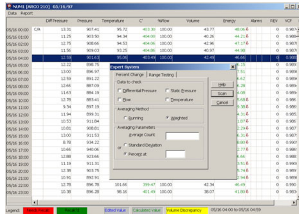
FIGURE 1. Statistical Expert System Data Scan
